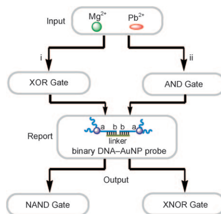
Figure 6. Representation of NAND and XNOR logic gates connected to binary DNA a-b -AuNP probes as colorimetric outputs. Each path is characterized by colorimetric and UV/Vis detection. The detailed schematic illustrations and results are given in the Supporting Information.
